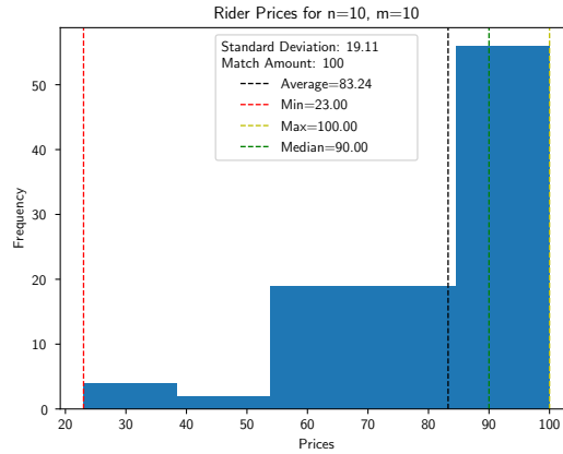
Figure 4: Rider Prices Distribution for n = m = 10
