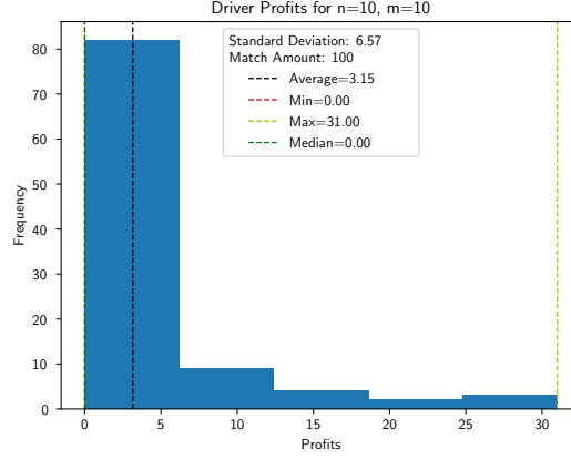
Figure 3: Driver Profits Distribution for n = m = 10
