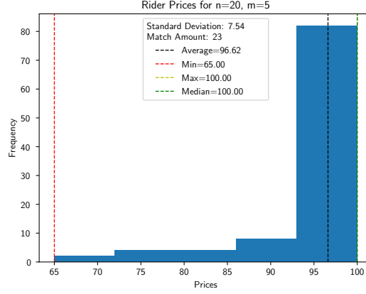
Figure 8: Rider Prices Distribution for 20 = n \gg m = 5
