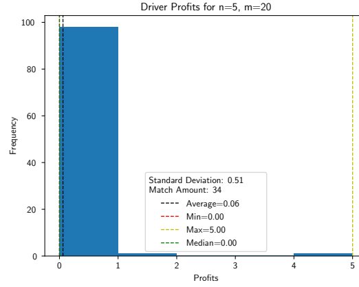
Figure 5: Driver Profits Distribution for 5 = n \ll m = 20
