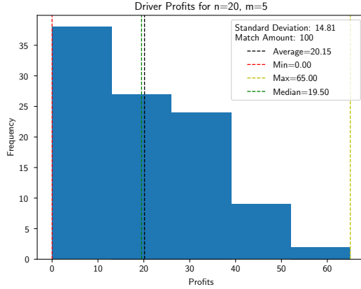
Figure 7: Driver Profits Distribution for 20 = n \gg m = 5
