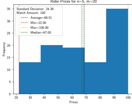
Figure 6: Rider Prices Distribution for 5 = n \ll m = 20
